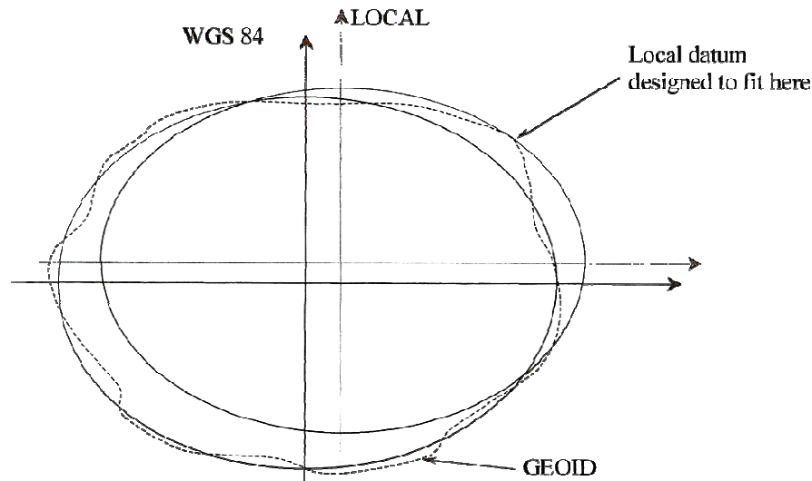
Fig. 2: Spheroid displacements
