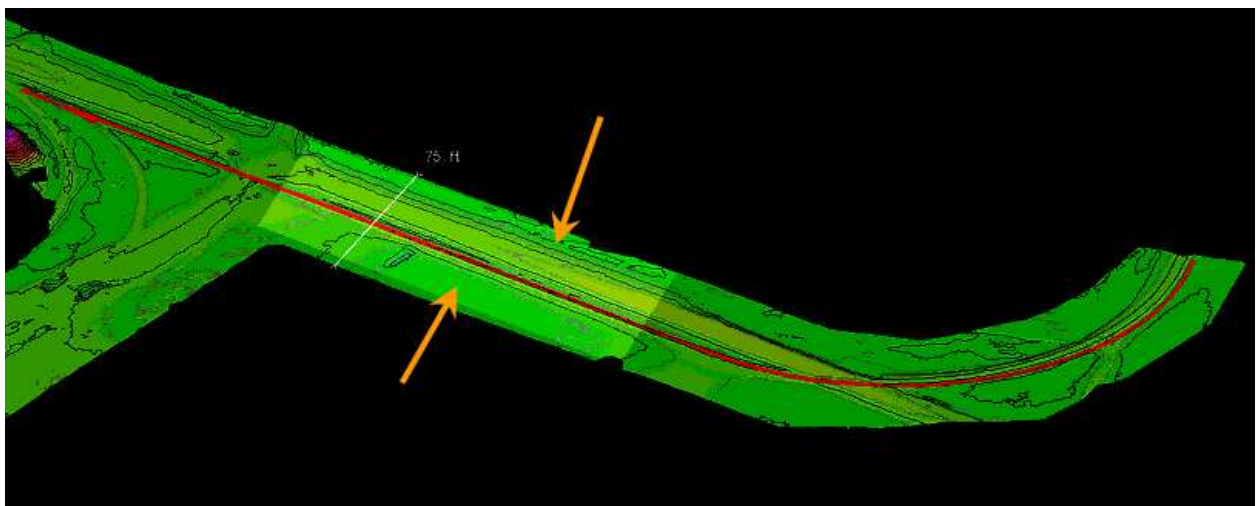
Figure 7: Triangulated Irregular Network (TIN) model with 1-foot contour lines showing a 75-foot corridor along a section of rail line
