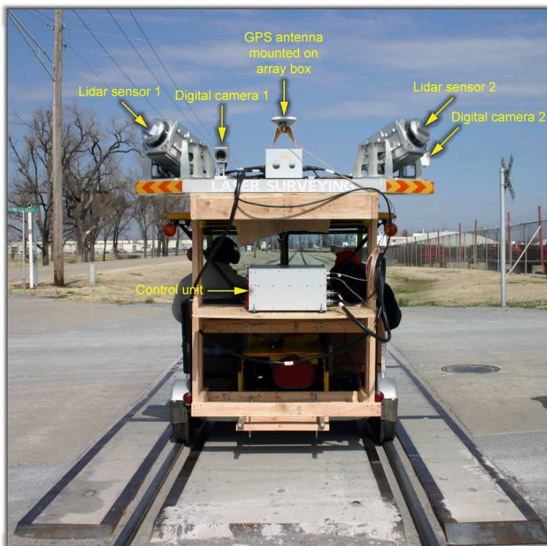
Figure 5: Lynx Mobile Mapper mounted on railway speeder
