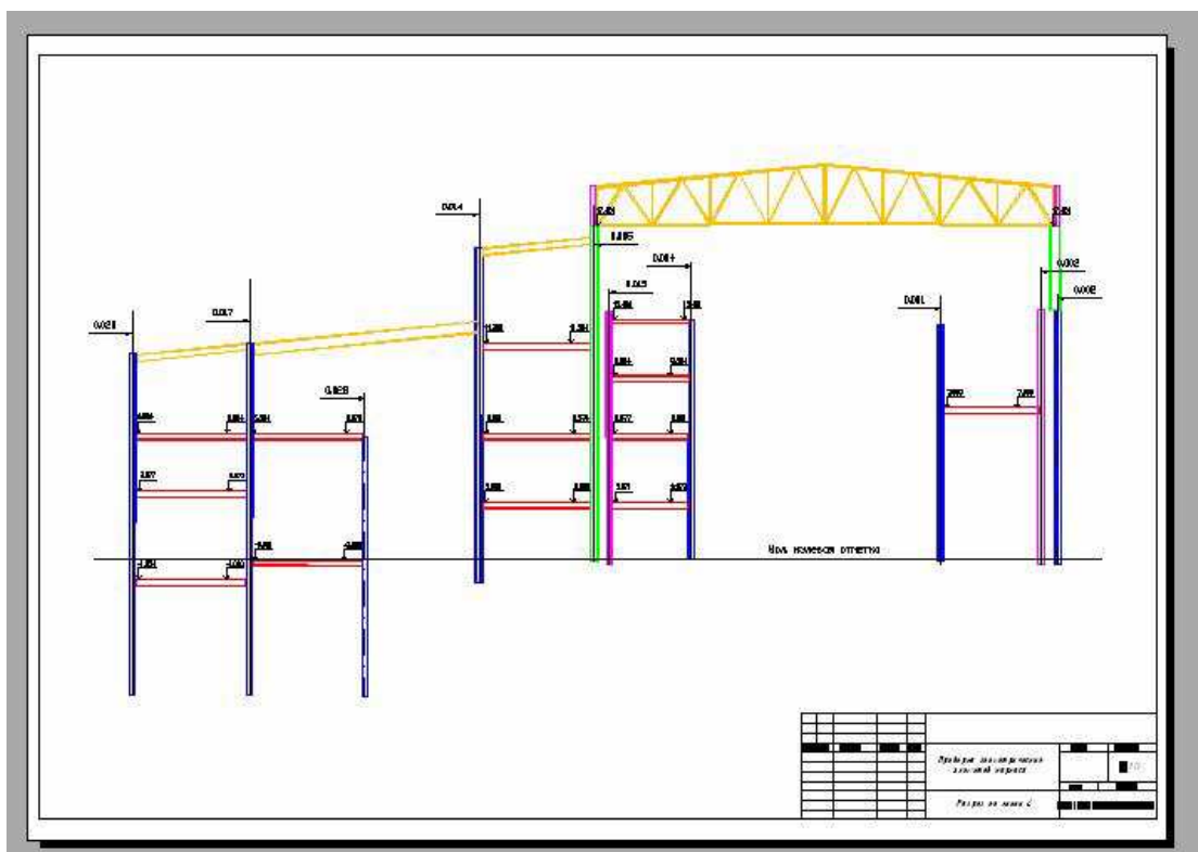
Figure 8: An approval drawing
