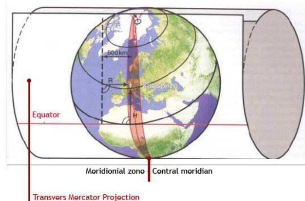
Fig. 1: UTM projection
