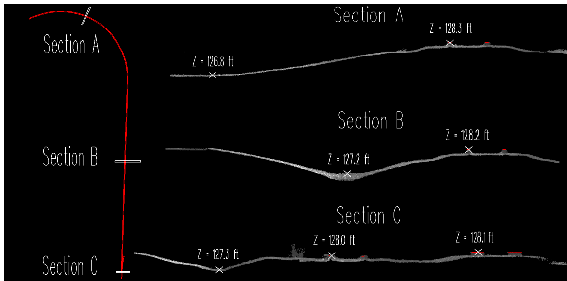
Figure 8: Cross-sections showing top rail elevation compared with lowest point along rail corridor.
