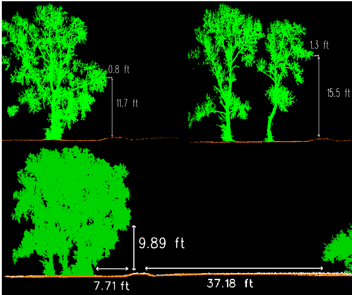
Figure 9: Various tree heights above top of rail, plus distance of trunk from top center of rail.
