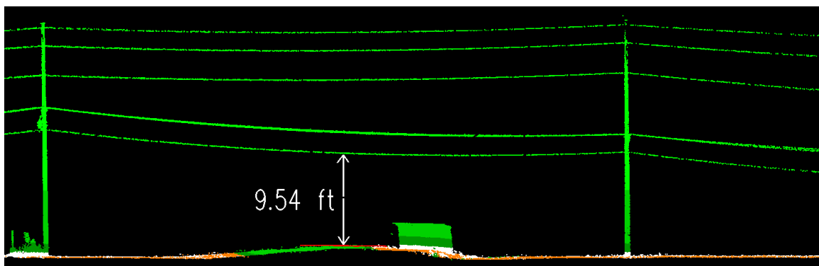
Figure 10: Height of overhead wires above top center of rail.
