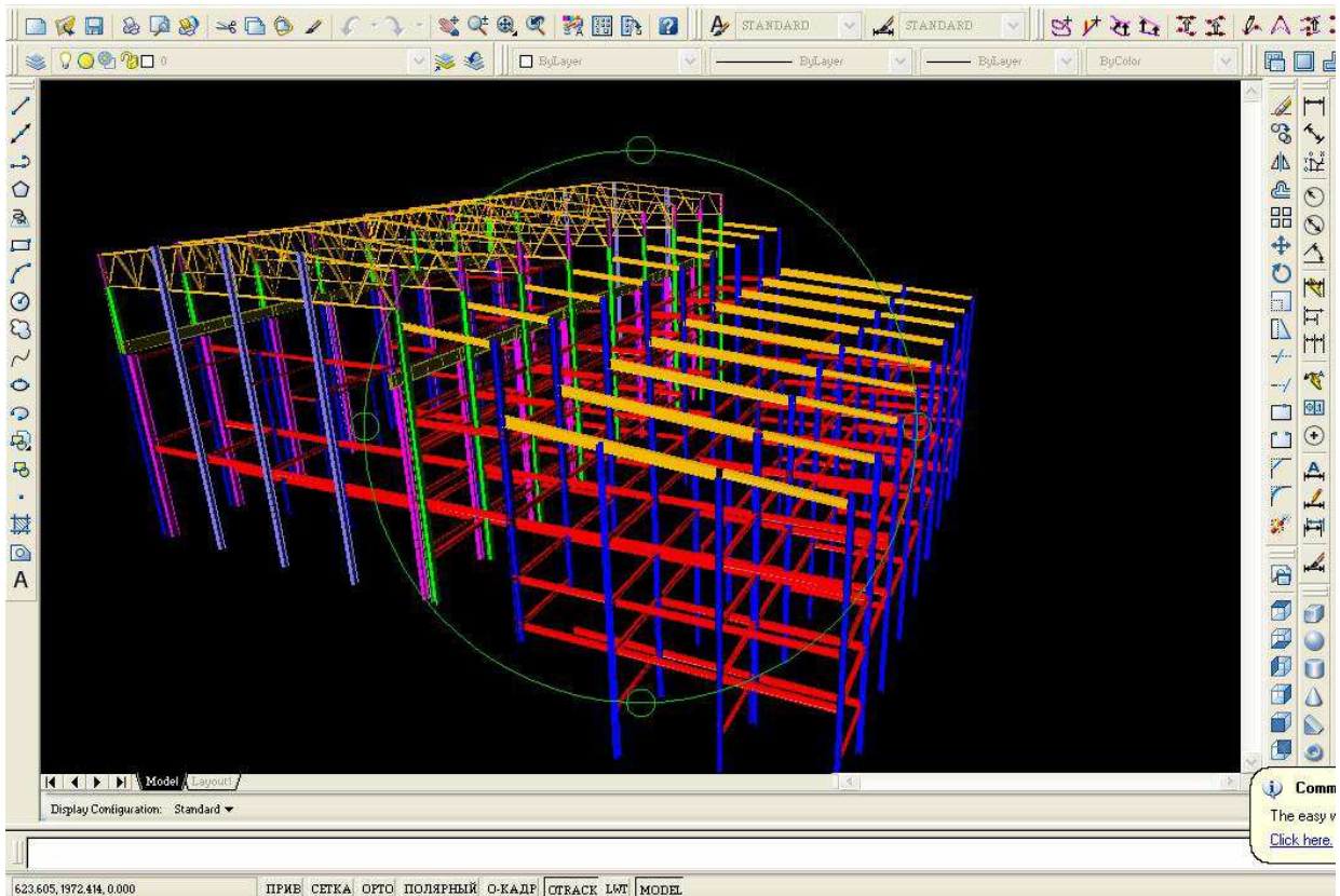
Figure 7: The distinguished load-bearing structures
